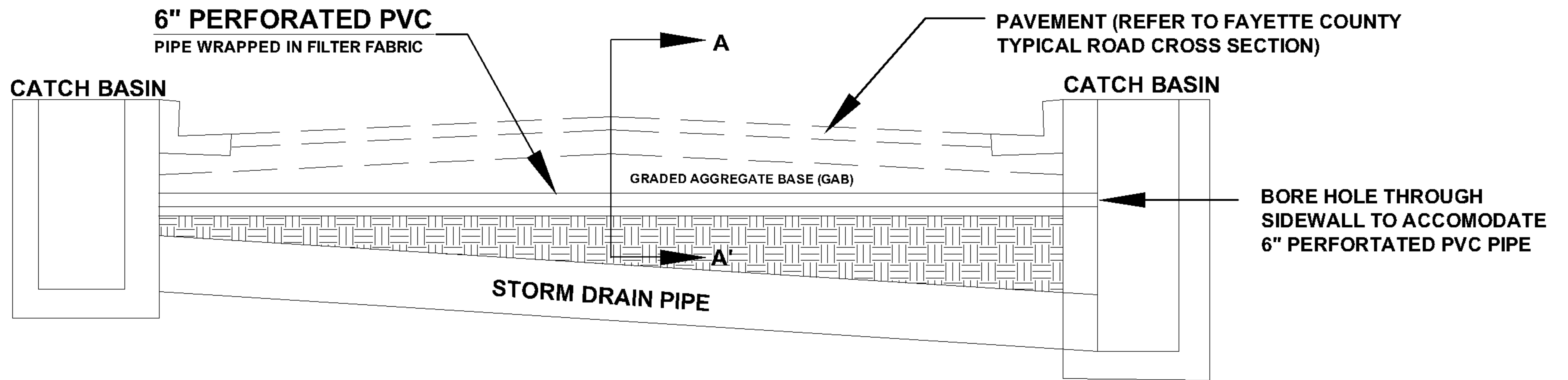
ROAD SECTION
