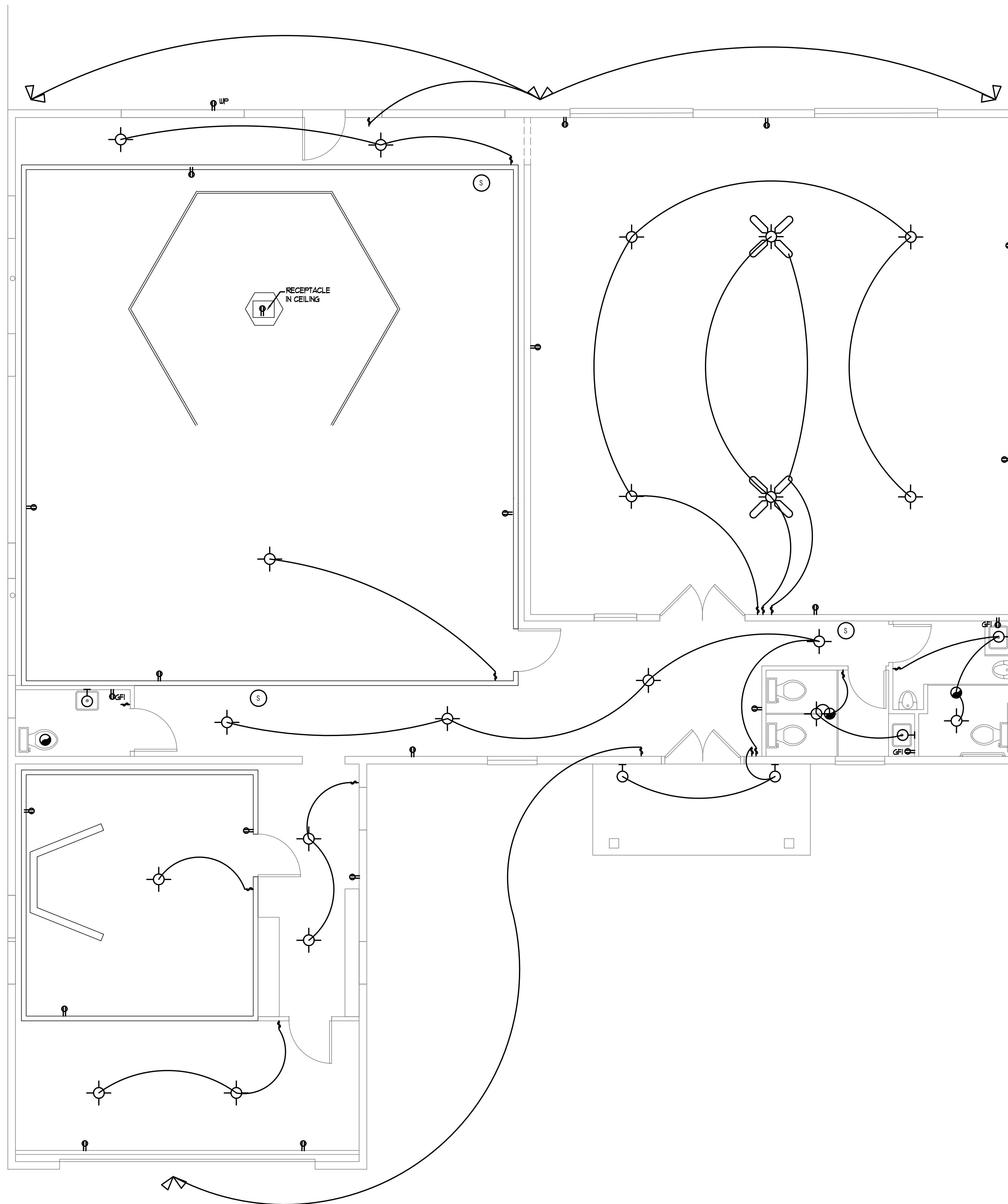
1 MAIN LEVEL ELECTRICAL PLAN
