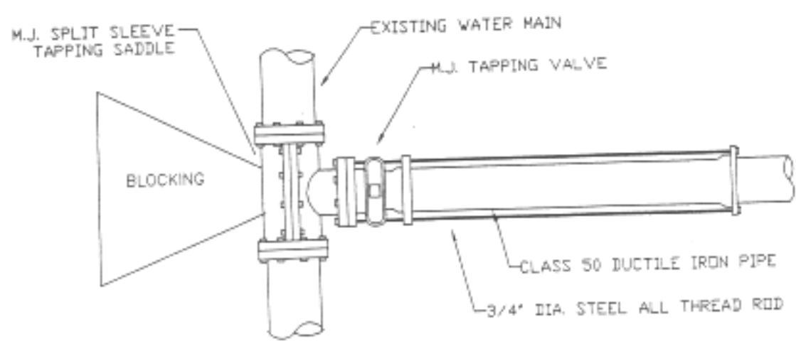
TYPICAL WET TAP INSTALLATION DETAIL
