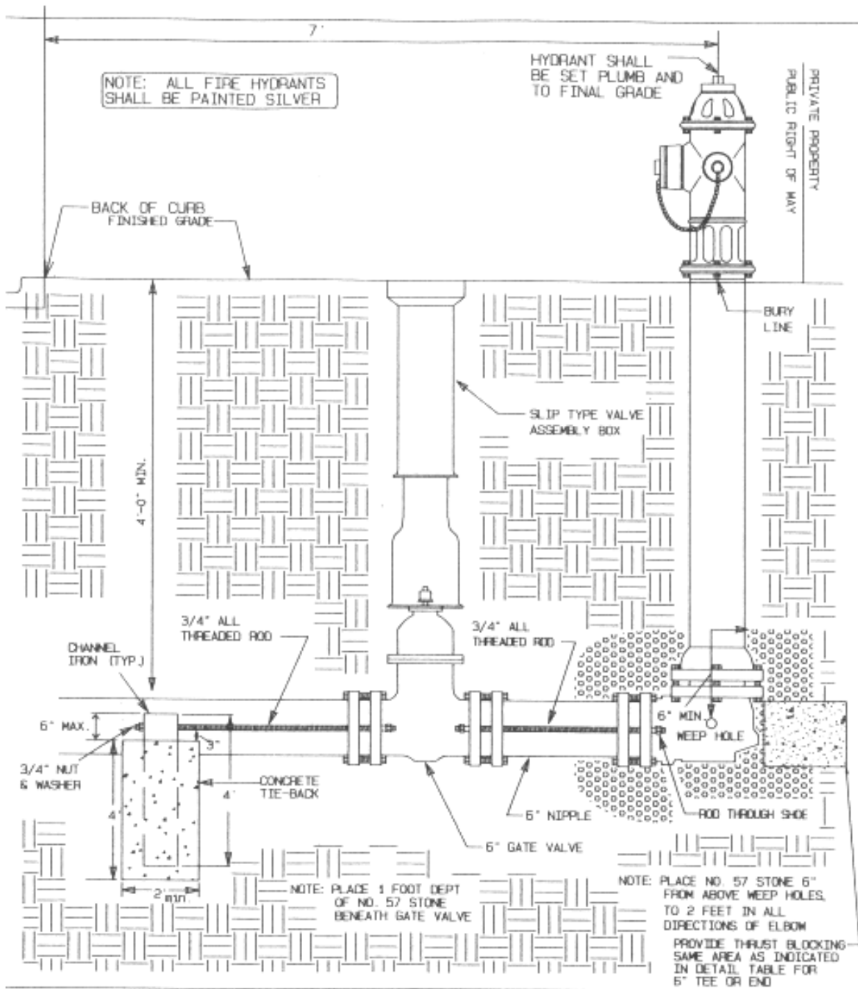
TYPICAL CUL-DE-SAC FIRE HYDRANT DETAIL
