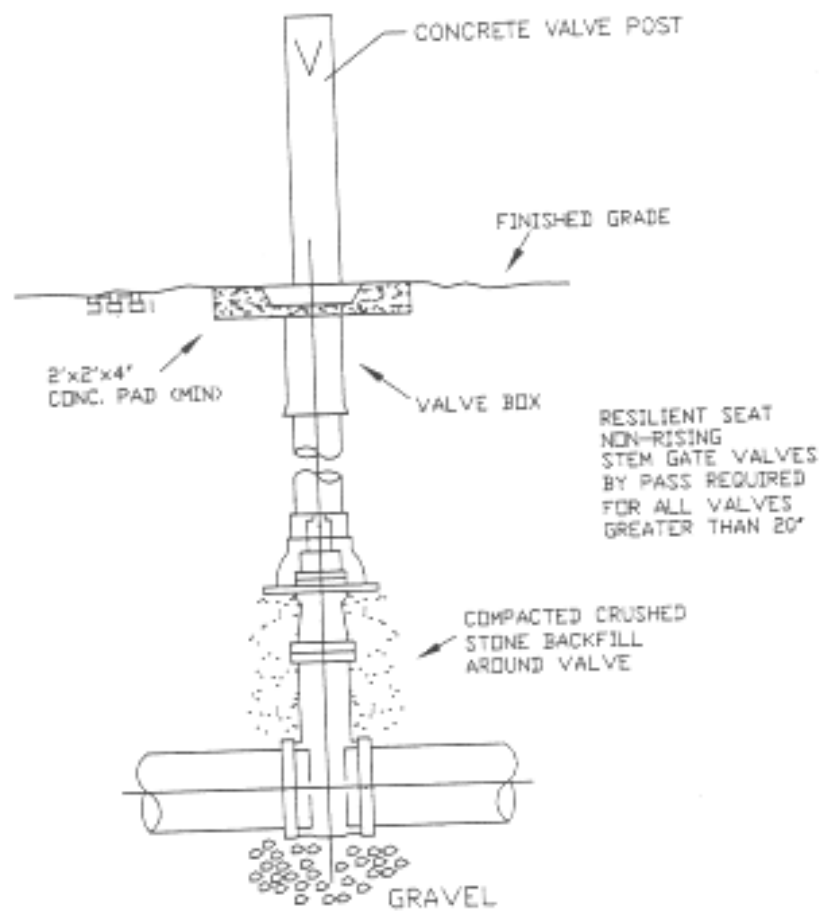
TYPICAL VALVE INSTALLATION
