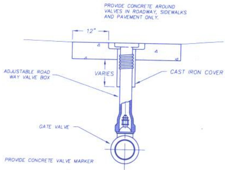
VALVE BOX DETAIL (NOT TO SCALE)
