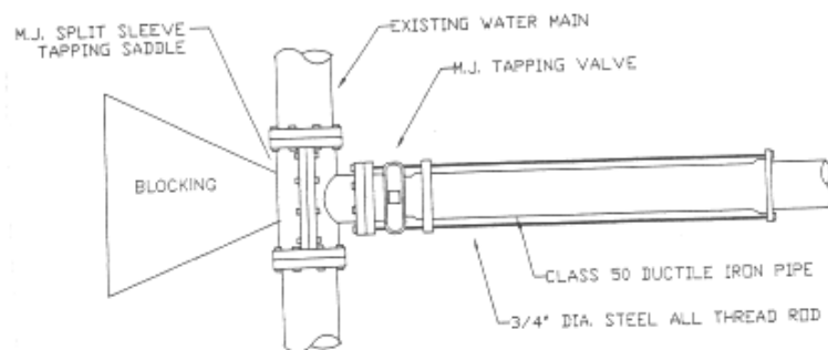
TYPICAL WET TAP INSTALLATION DETAIL
